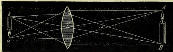
Real inverted image formed by convex lens.
